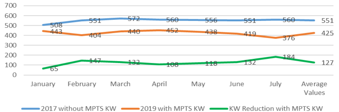
KW Reduction Tracking at Rayo Plant with MPTS compared to the year without MPTS technology
