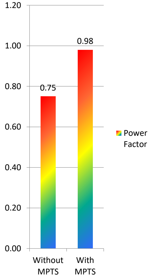
Power Factor
