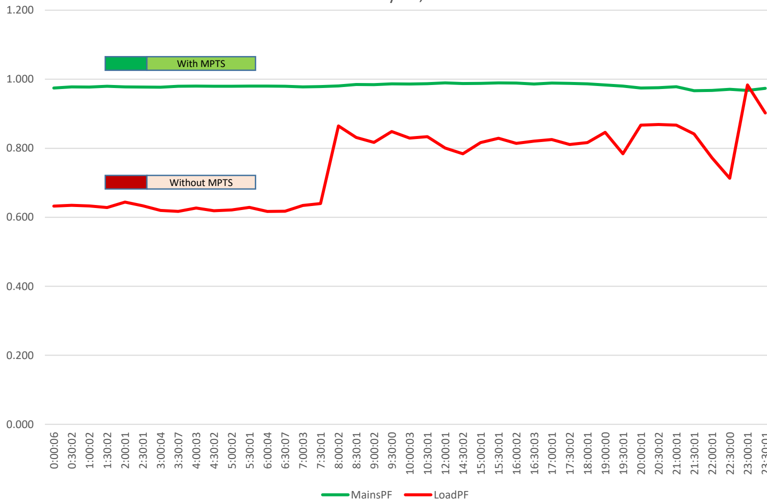
Power Factor - on 800 Amp Panel January 22, 2018
